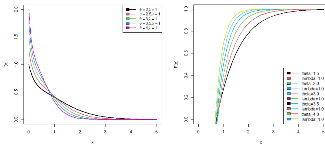
Figure 1. Pdf and Cdf plot of the New distribution (MEGD)
