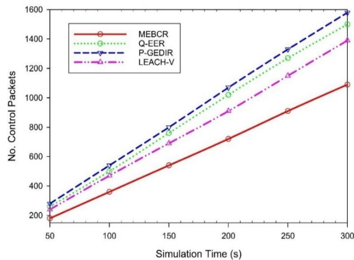
Figure 3. Routing Overhead
