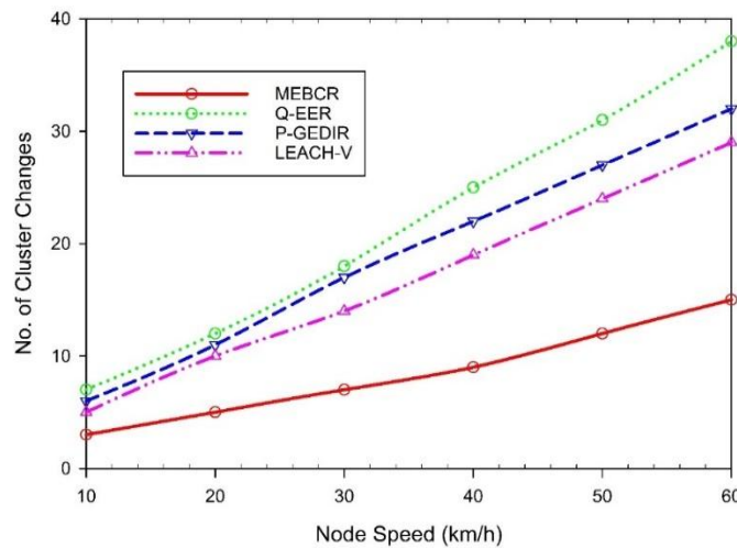
Figure 6. Cluster Stability
