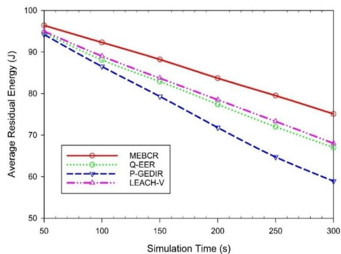
Figure 4. Energy Efficiency
