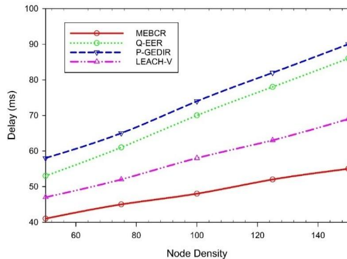
Figure 2. End-to-End Delay
