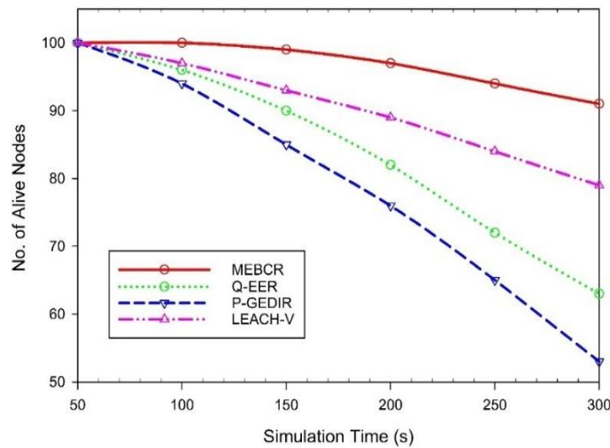
Figure 5. Network Lifetime
