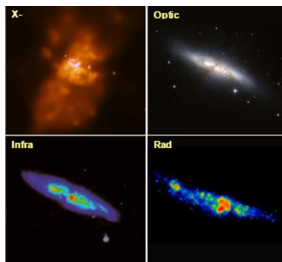
Figure 3: The images showcased offer diverse viewpoints of the star-forming activities happening within M82, each captured at different wavelengths. The sources for these images are as follows: X-ray image -
